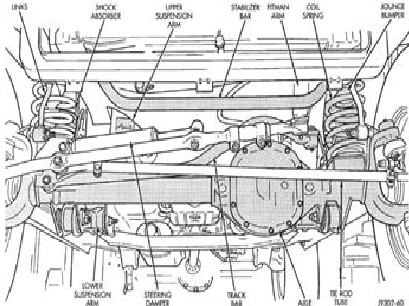
Fig. 1 Front Suspension
