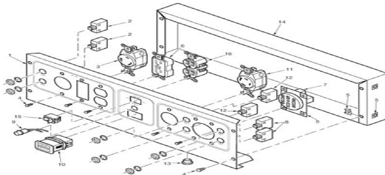
Figure 47 - Repair Parts Illustration for Model 3WY47 Control Panel
