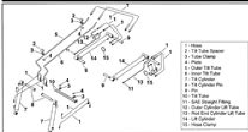
Fig. 9-30 Exploded view of LiTTit Self-Leveling Hydraulics - Lift Arm - SX Models.
