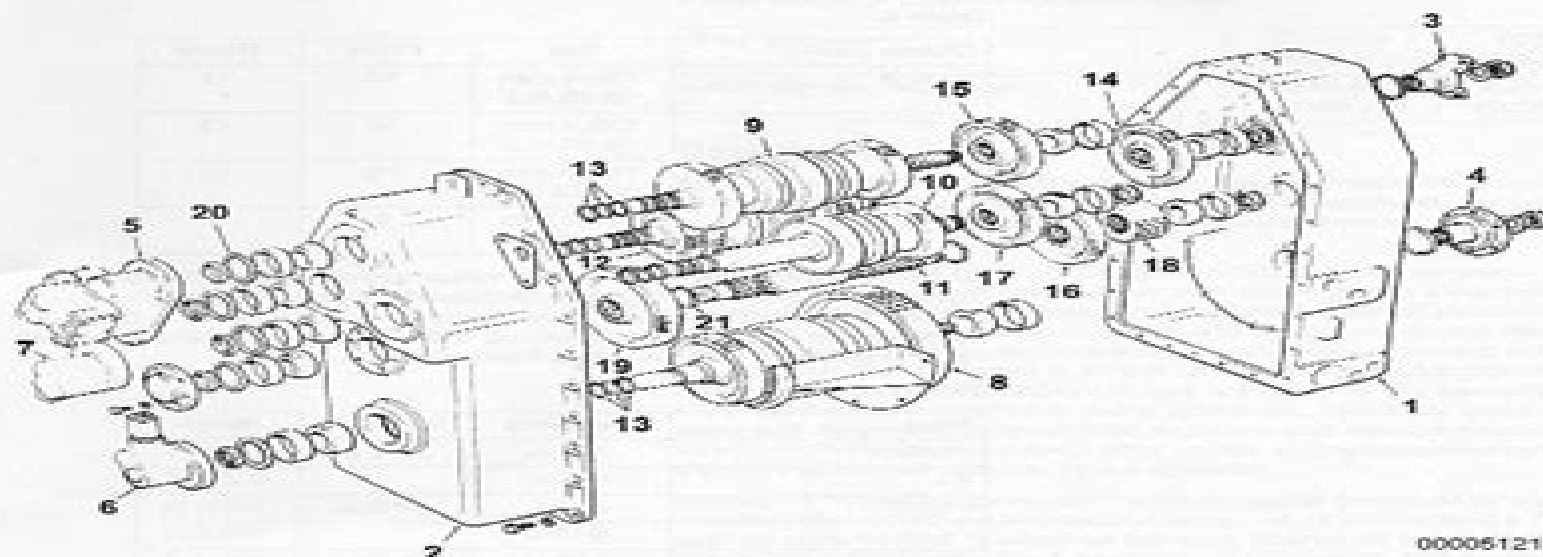
Fig. 25 8400 Transmission exploded assembly
