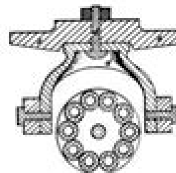
FIG. 5. SECTION THROUGH BARREL AND MOUNTING BRACKET, AND MOUNTING BLOCK.
