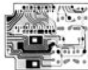
Physical Layout of Mounting Side
