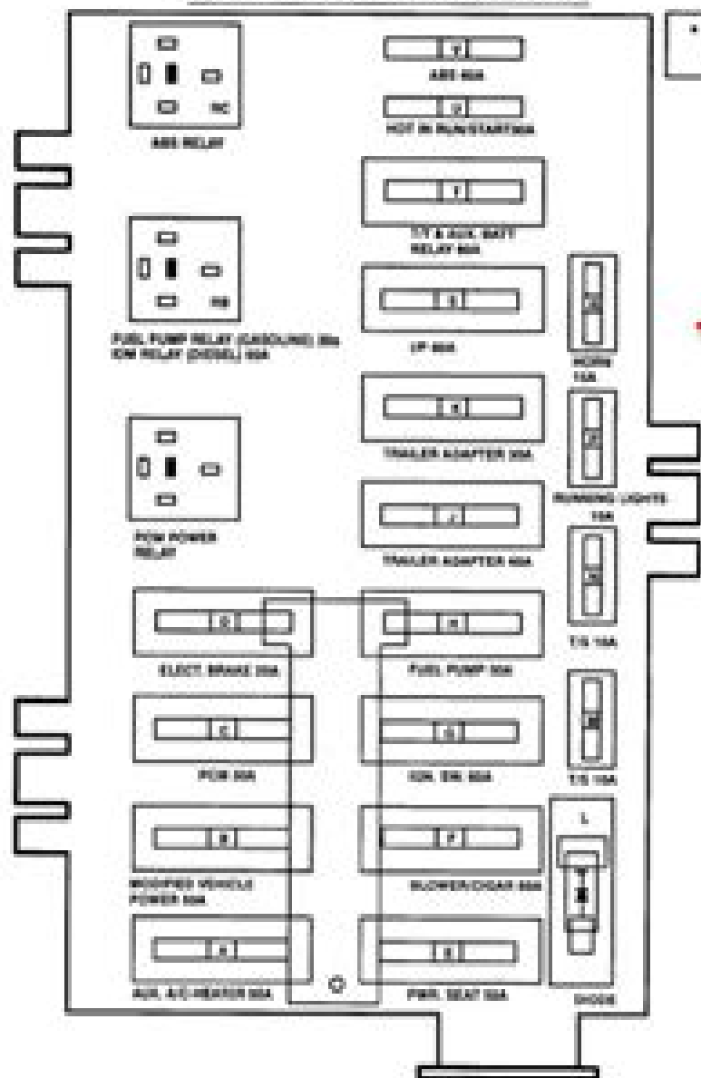
ENGINE COMPARTMENT FUSE PANEL
