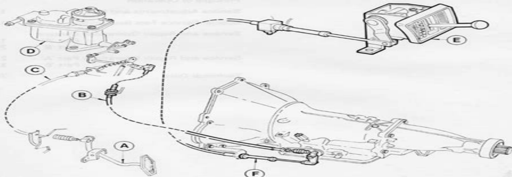
Fig. 1. Automatic transmission operating system
