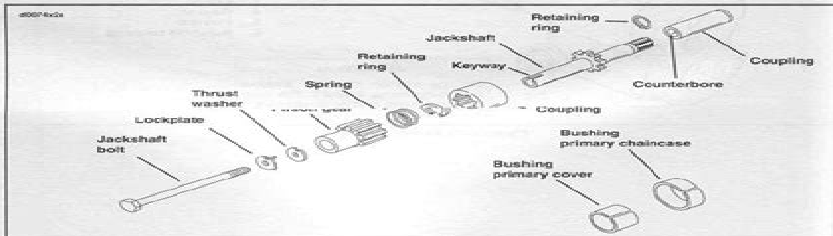
Figure 5-28. Starter Jackshaft
