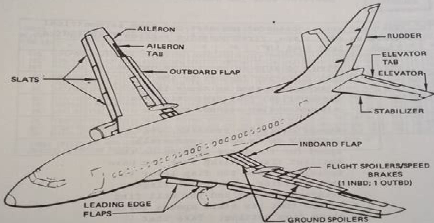
CONTROL SURFACES
