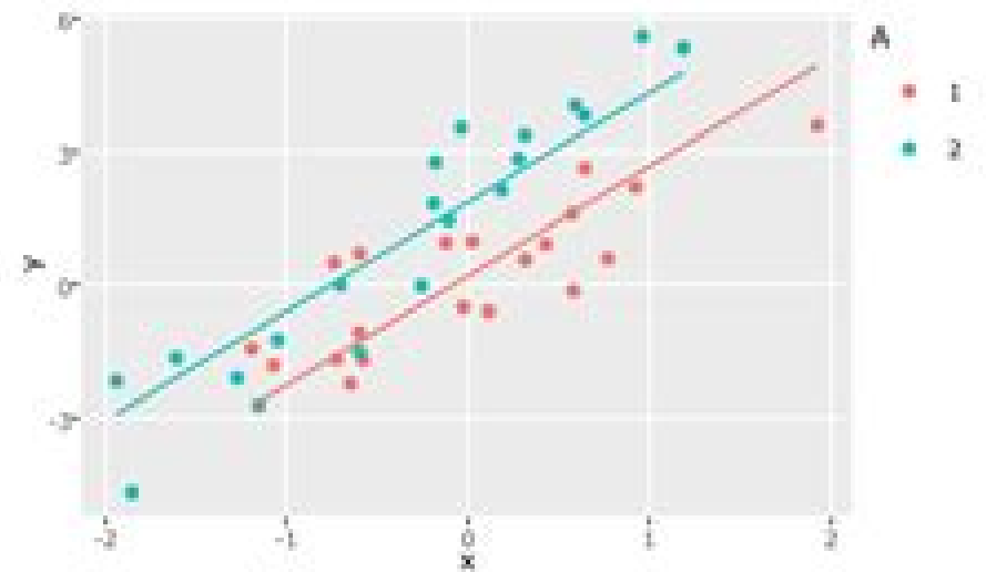
Constraining Slope with stat_smooth
