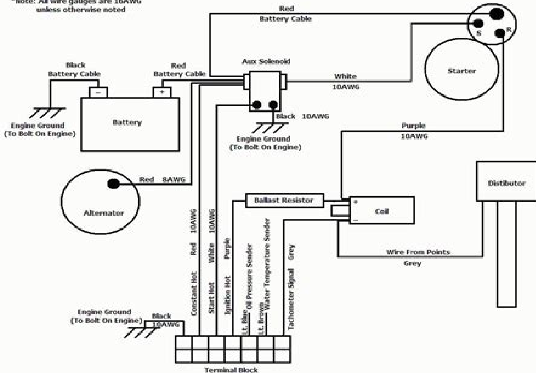
Typical Jet Boat Engine Harness 1-wire alternator, points ignition
