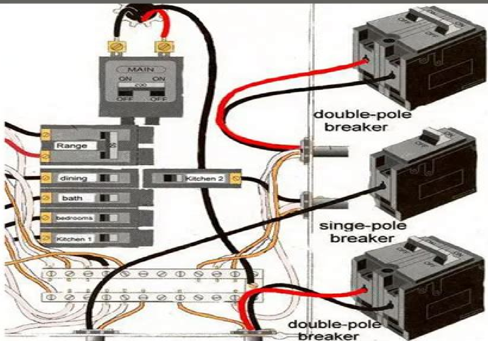
Different types of breakers and common breaker labelling
