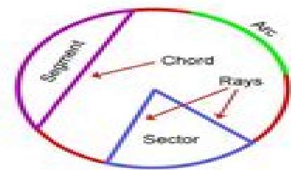
Parts of a Circle
