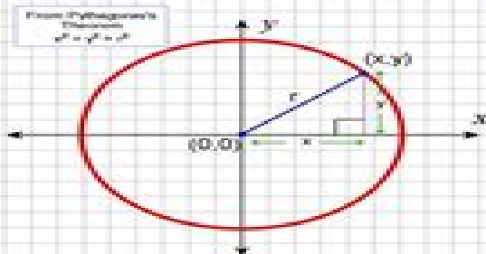
Equation of a Circle With Centre at the Origin
