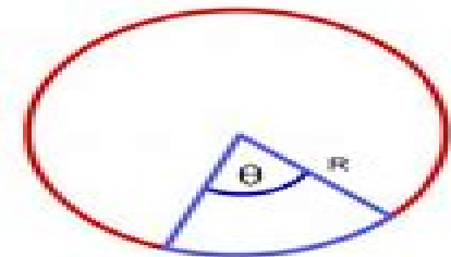
Area of a Sector = \theta R^2/2
