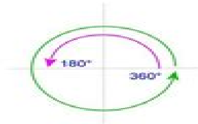
360 Degrees in a Full Circle
