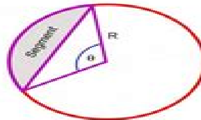
Area of a Segment = R^2/2 (\theta - \sin \theta)
