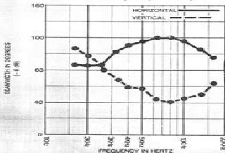
FIGURE 3 Beamwidth vs Frequency — HT94 Whole Space (Anechoic)
