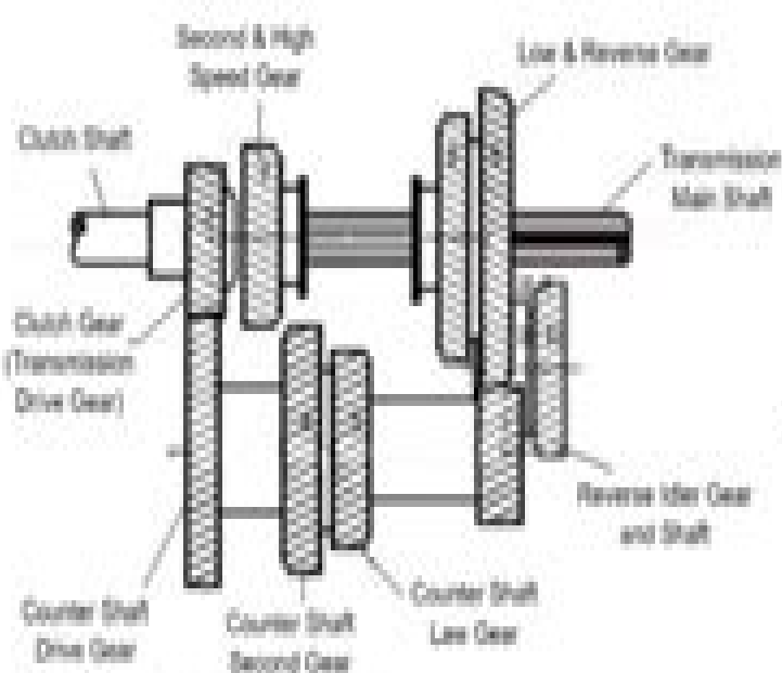
Sliding Mesh Gearbox
