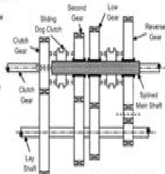
Constant Mesh Gearbox
