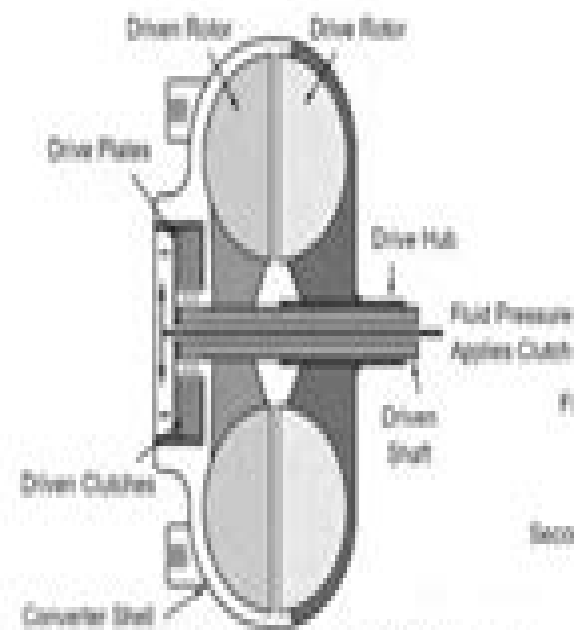
Hydraulic Torque Converter
