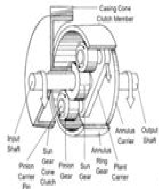
Epicyclic Gearbox
