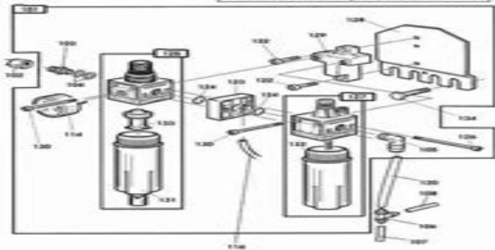
Figure 4 Bead Breaker
