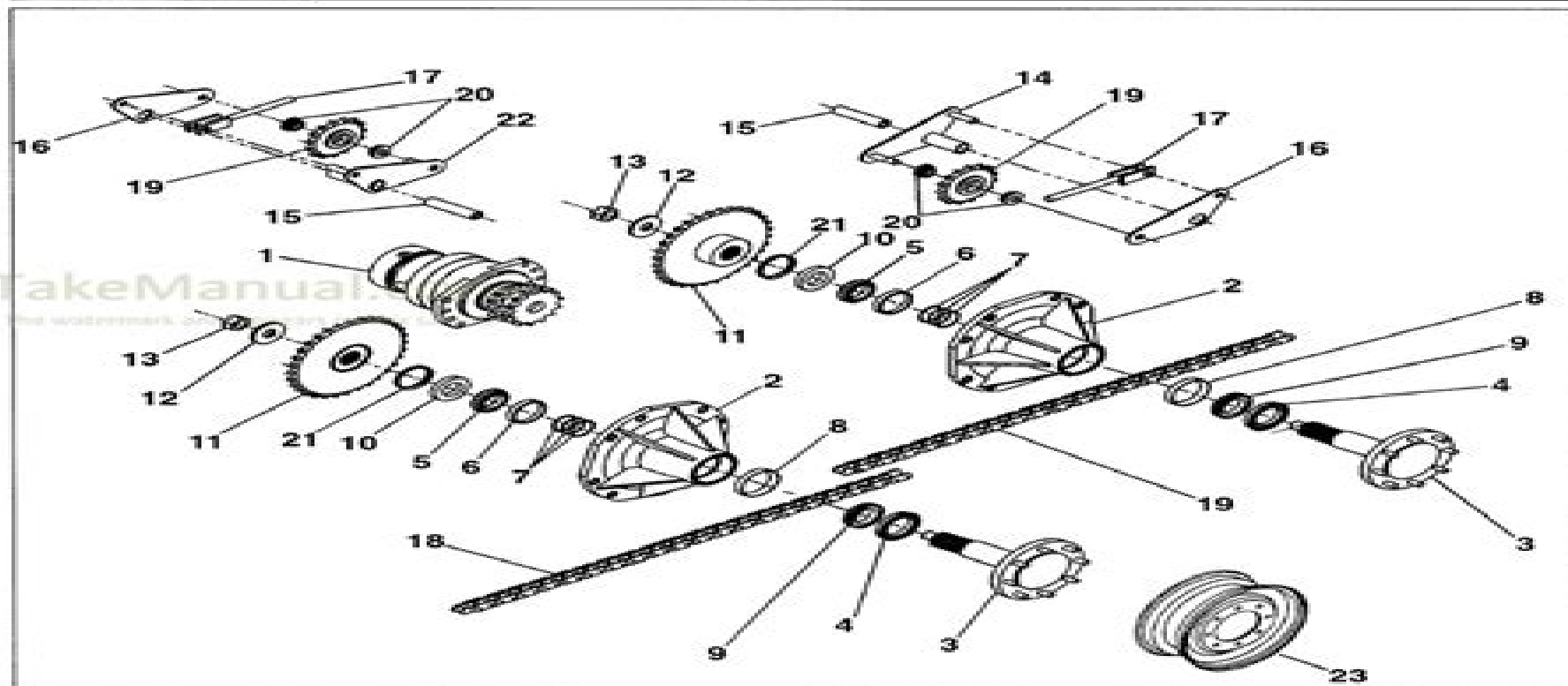
Fig. 5-1 Exploded view of Wheel Drive components (left side shown, right side typical).
