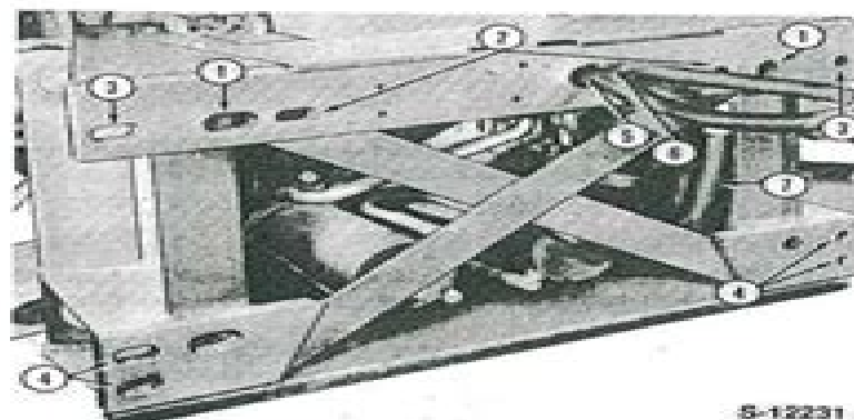
Figure 71 Backhoe Hoses Storage Position
