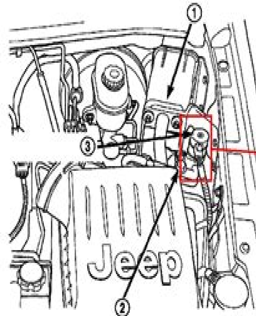
Fig. 15 EVAP Canister, EVAP Solenoid, LDP Test Port Locations
