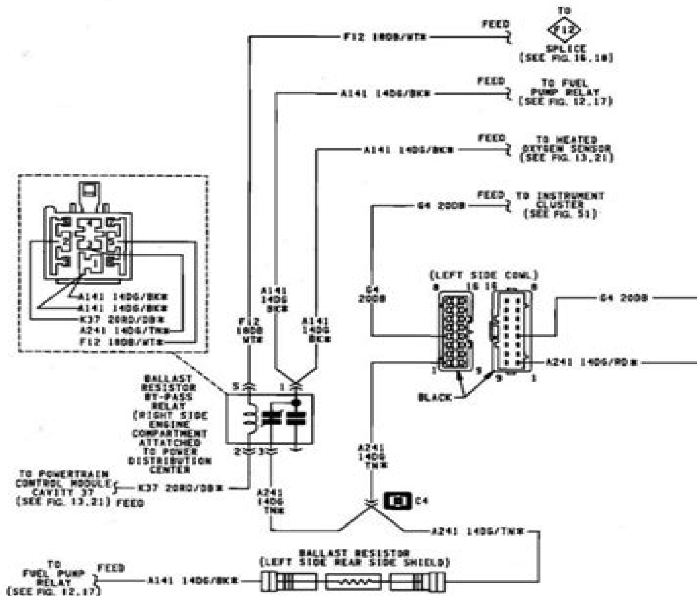
Fuel Tank System
