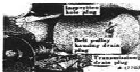
Illust. 10 - Drain Plugs
