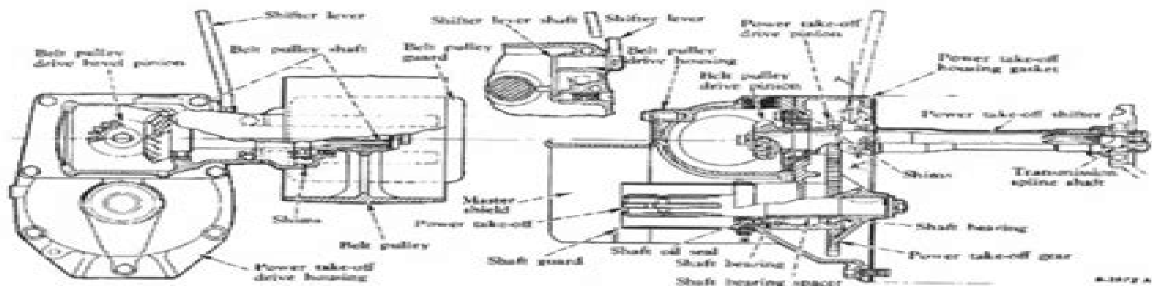
Illust. 12 - Belt Pulley and Power Take-off Assembly
