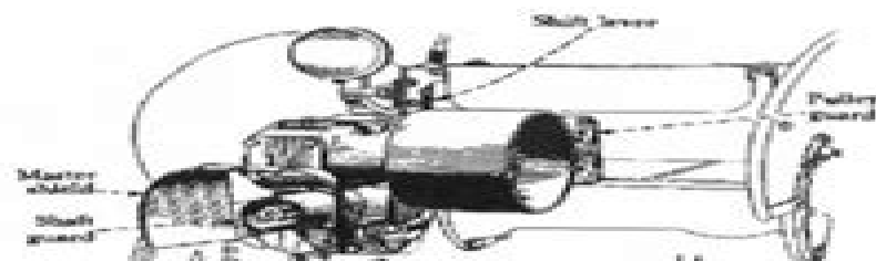
Illust. 11 - Belt pulley and Power Take-off Assembled on Tractor
