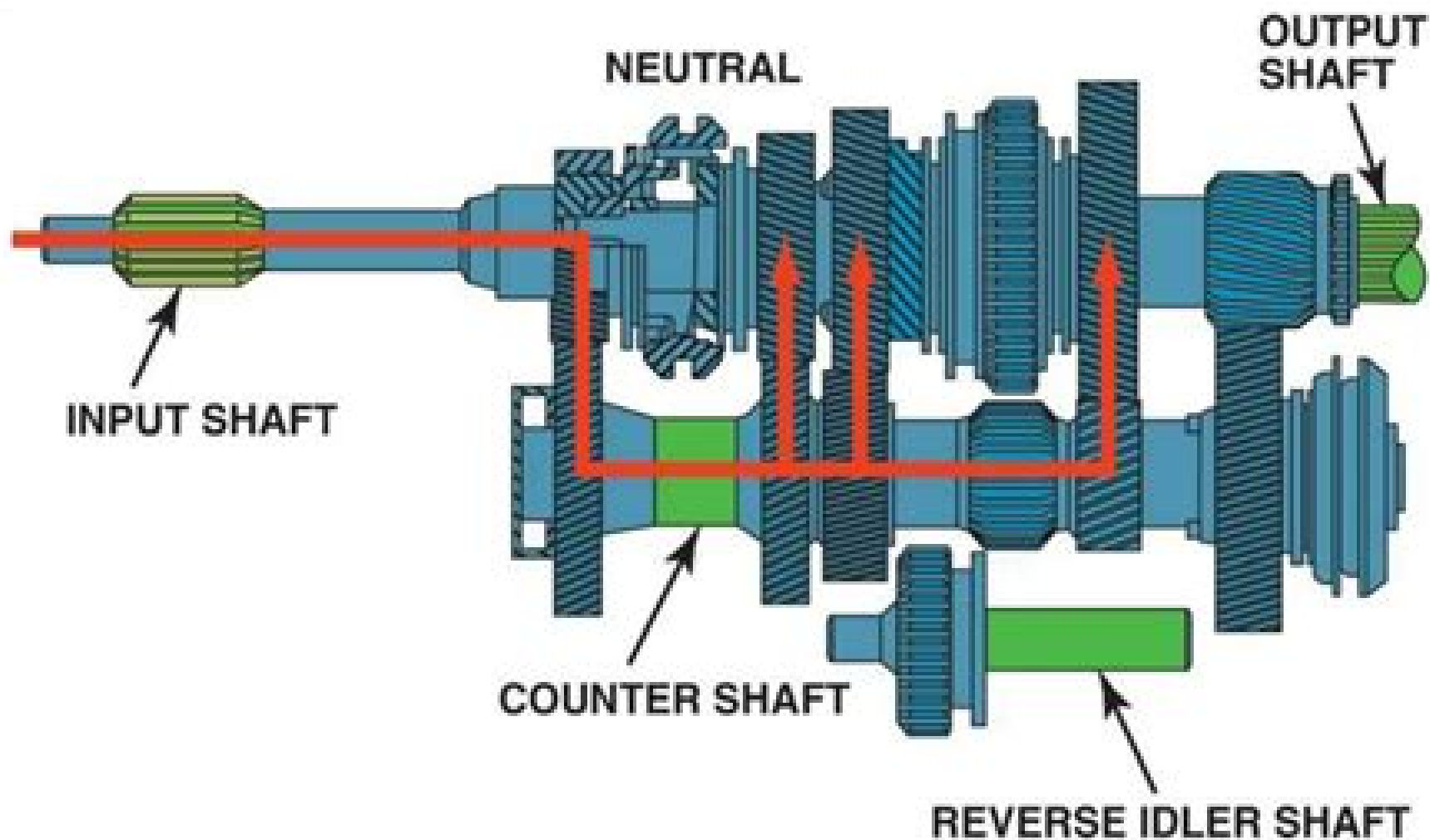
Figure 122-24 In neutral, the input shaft and the countershaft are rotating if the clutch is engaged (clutch pedal up), but no torque is being transmitted through the transmission.
