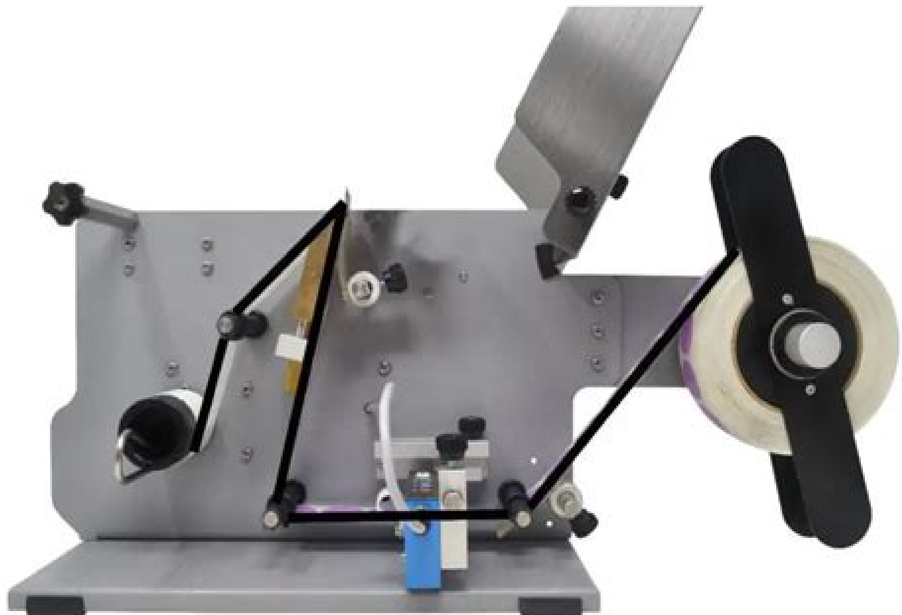
Figure 6 – Label Feeding Diagram Highlighted:
