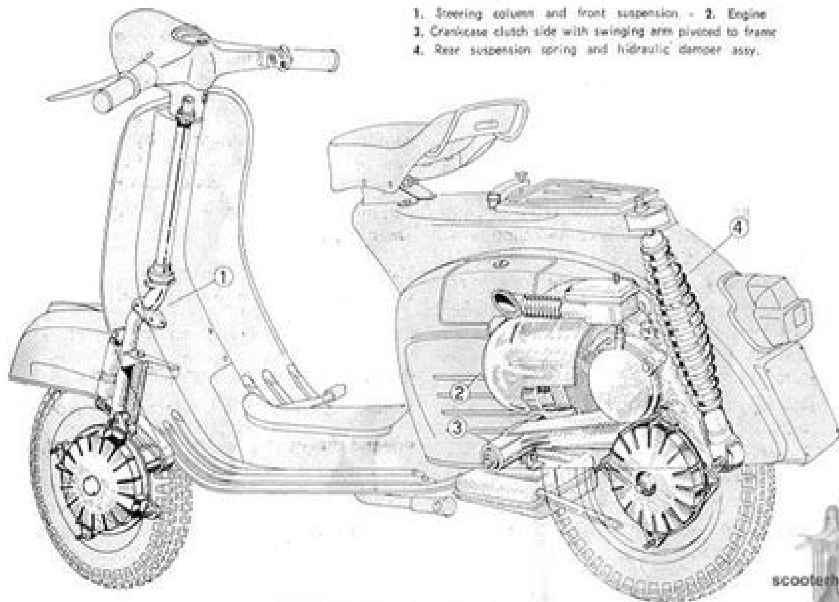
Fig. 20 - Installation of engine and suspension
