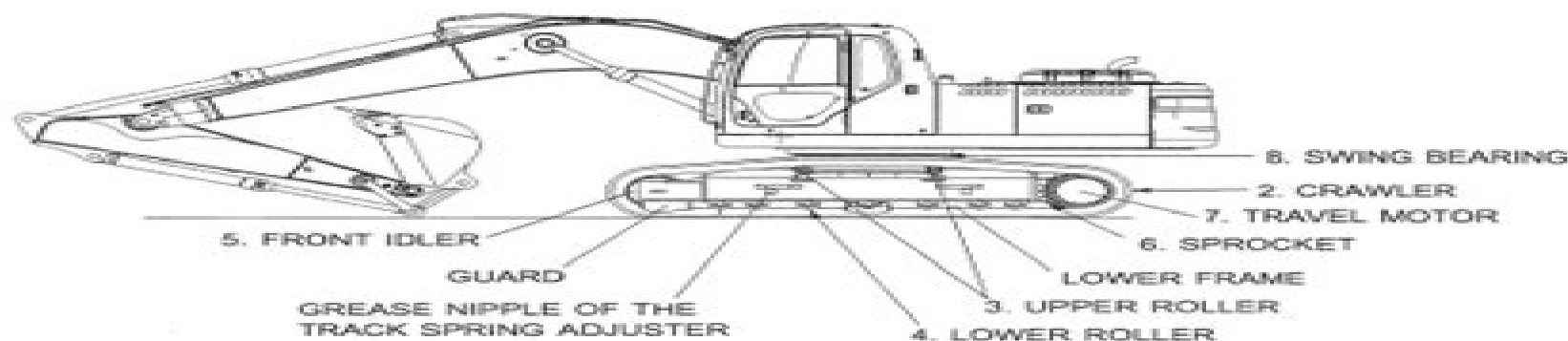
Fig. 34-1 Designation and location of undercarriage
