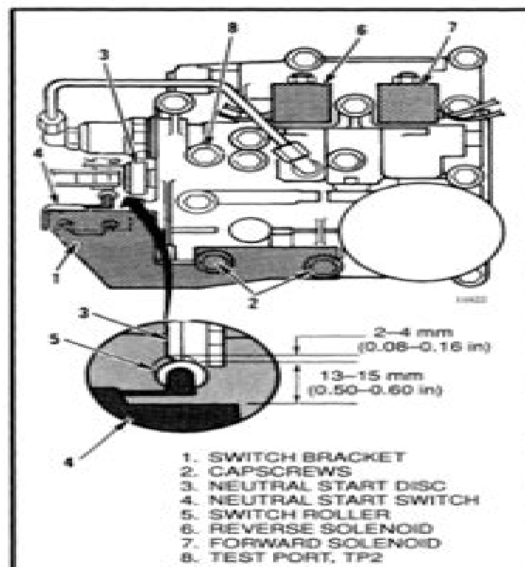
FIGURE 11. ADJUSTMENT, NEUTRAL START SWITCH (MONOTROL ONLY)
