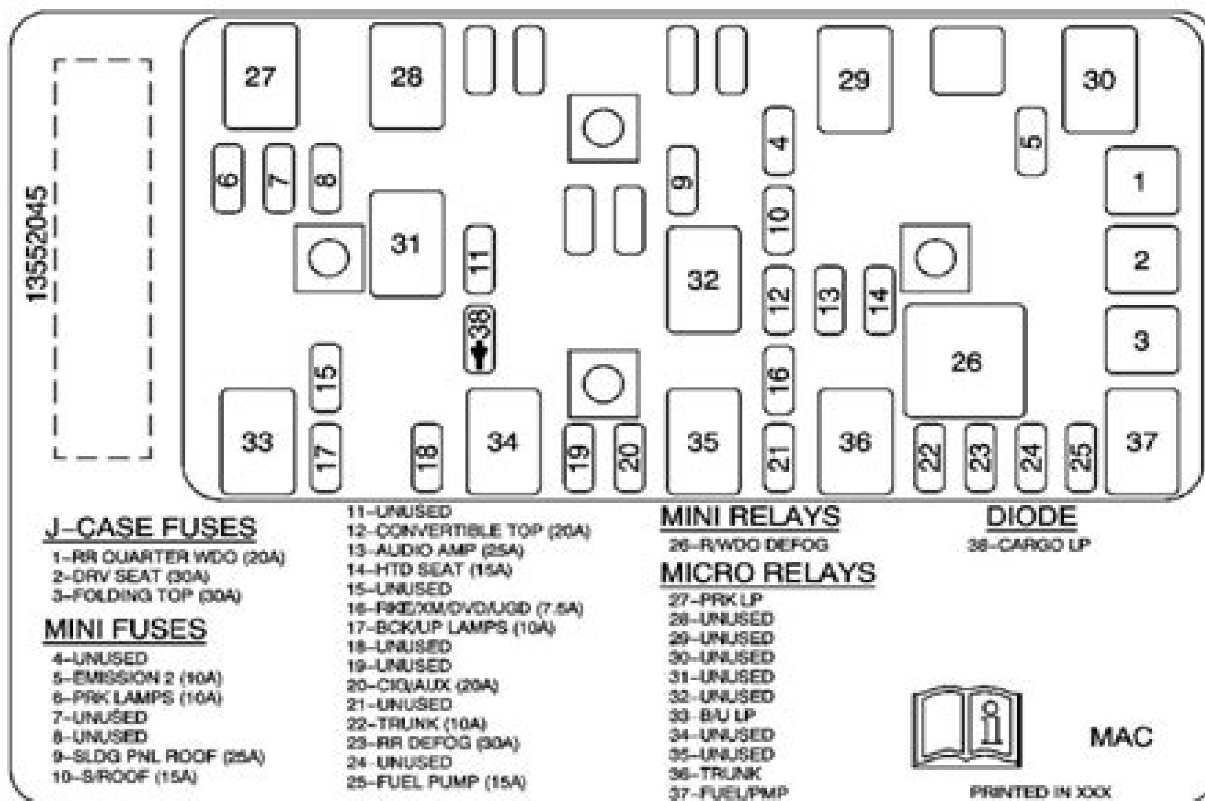
Fig. 9: Identifying Rear Fuse Block Components
