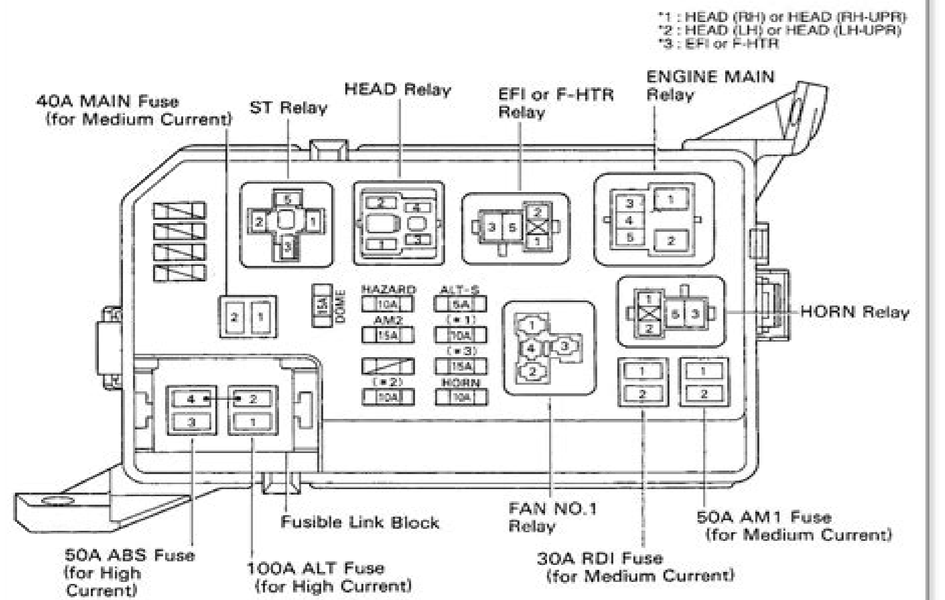
Fig. 15: Identifying Engine Room J/B Components
