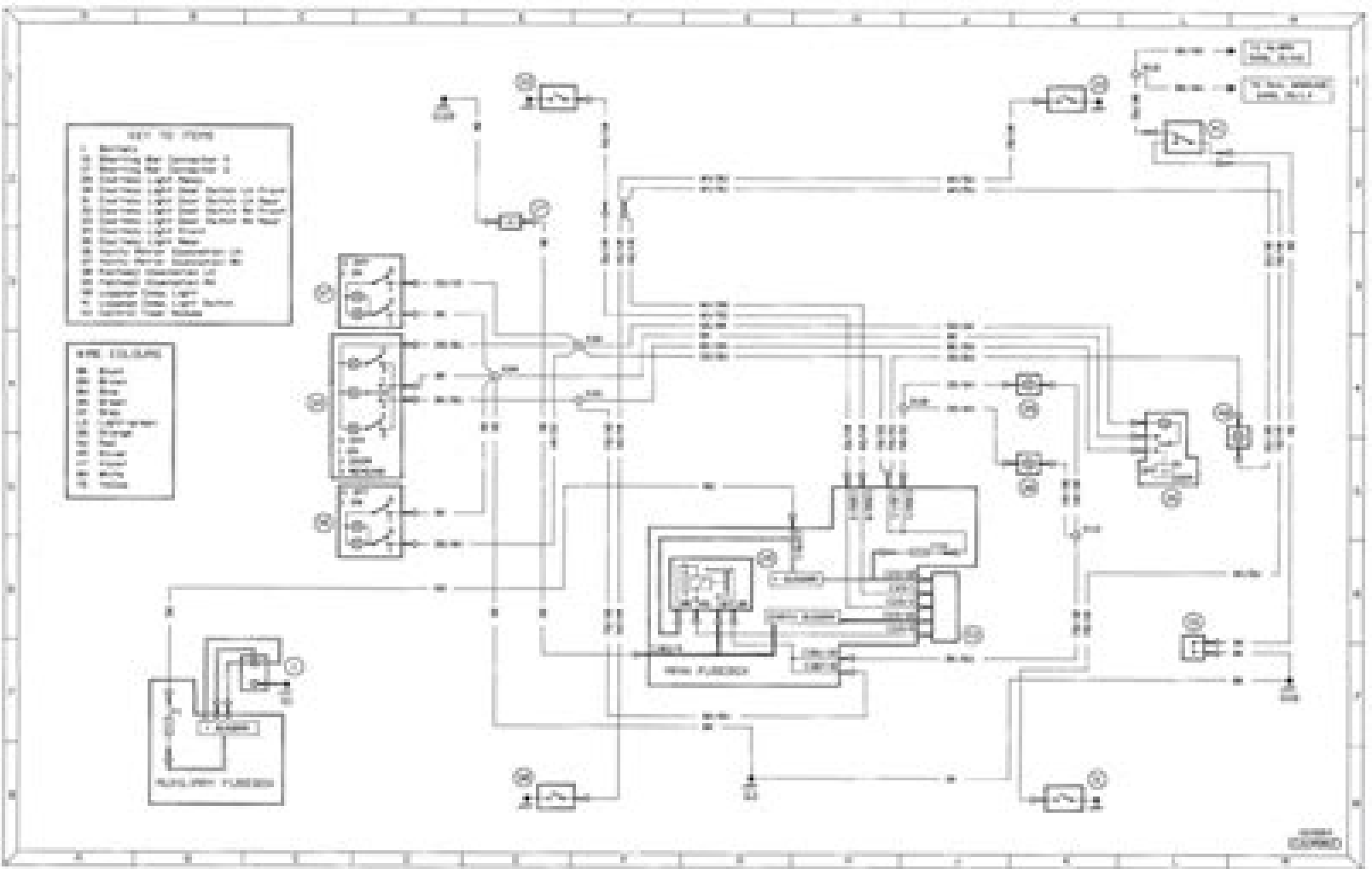
Diagram 13: Interior lighting - front and rear courtesy, footwell and luggage compartment lights
