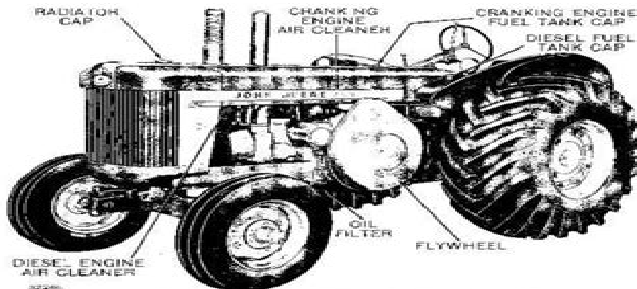
Figure 16-5-2—John Deere "820" Series Diesel Tractor—Flywheel Side
