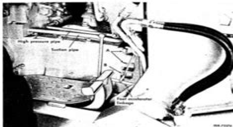
Illustr. 5. Right side view of tractor.
