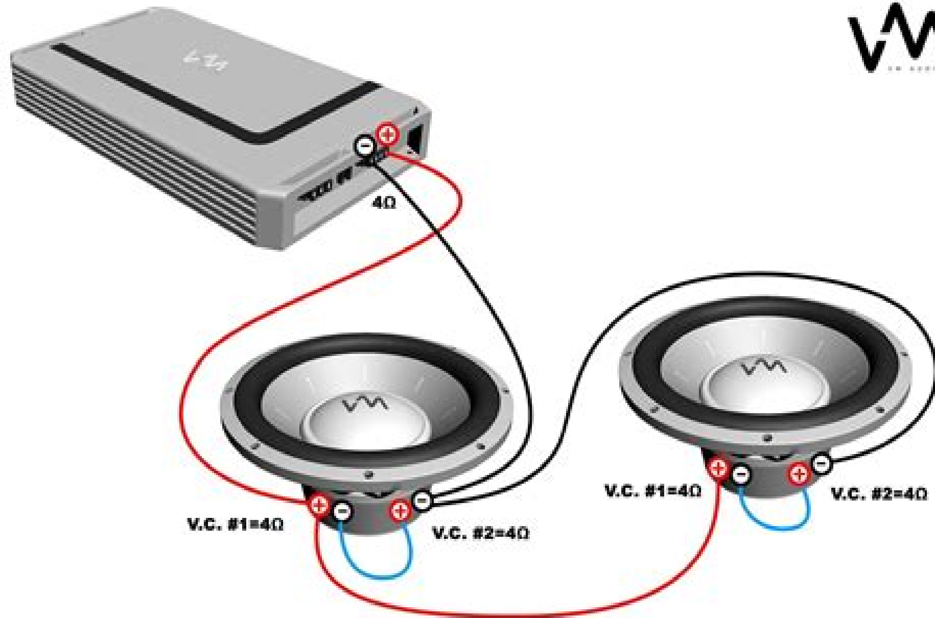
TWO 4Ω DVC SUBS, BRIDGED 2-CHANNEL AMP: 4Ω LOAD
