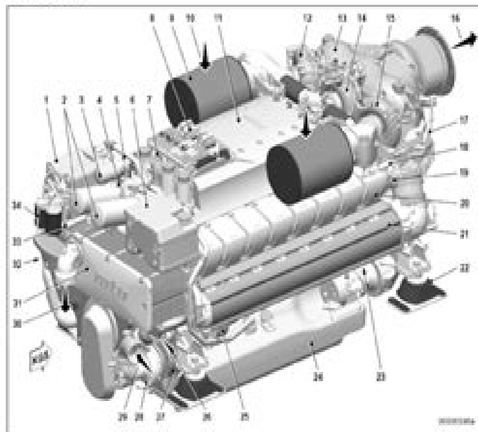
Engine layout
