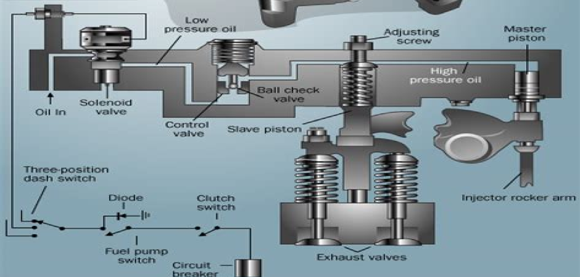
Cross Section
