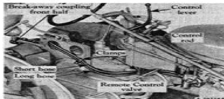
Illustration 93 Control valve hoses and control lever.
