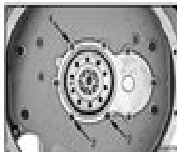
Figure 411 Rear of seal carrier bolts (stripped chassis)
