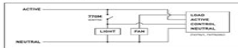
Figure 2. Fan delay timer
