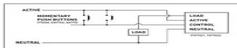
Figure 1. Normal wiring diagram
