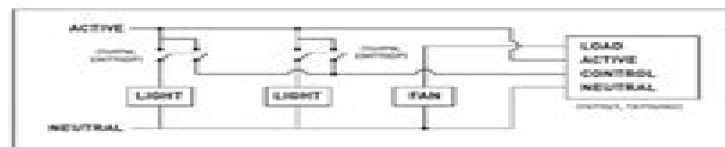
Figure 3. Fan delay timer with multiple lights
