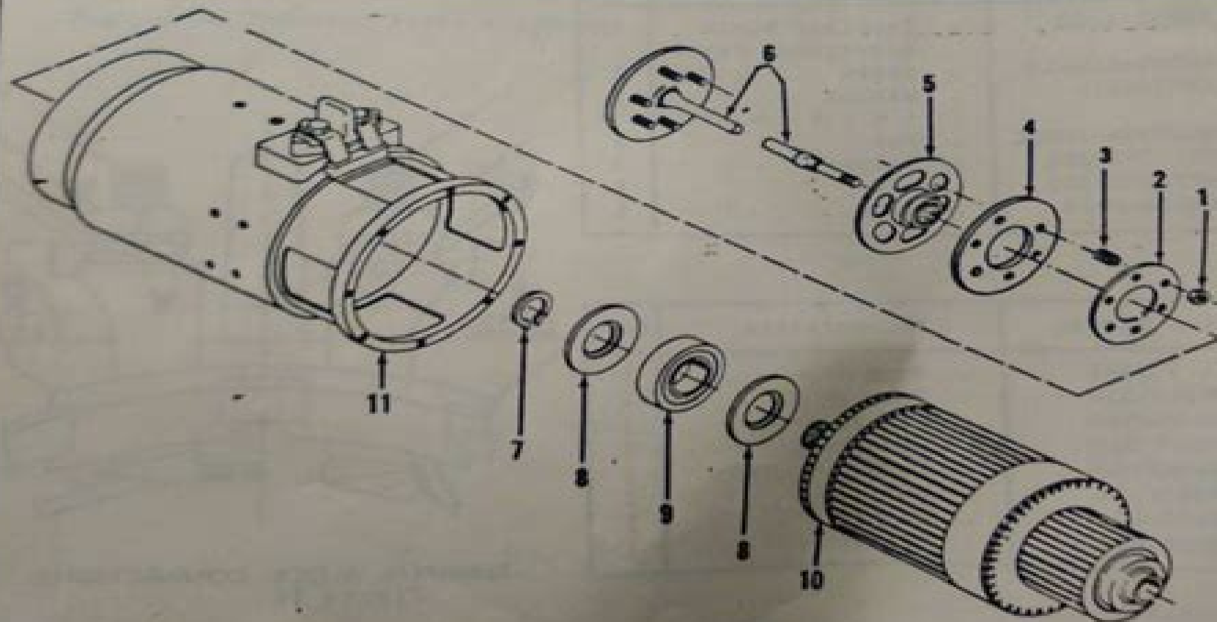
Figure 17. Partial Exploded View Of Starter Generator 23035-006
