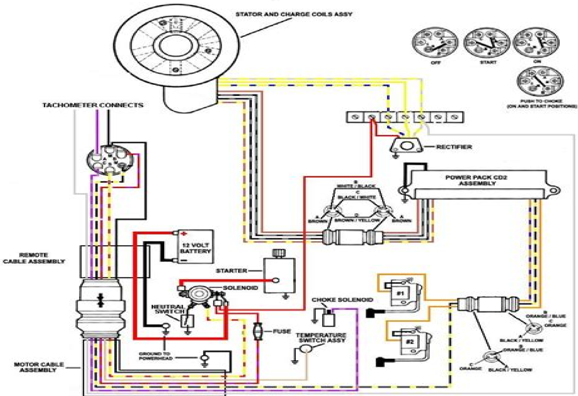
WIRING DIAGRAM
