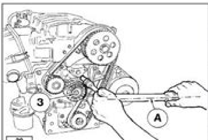
Camshaft timing - Belt Tightening and Fastening
