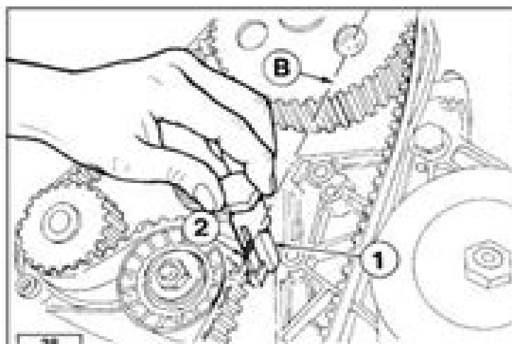
Camshaft timing - Belt tightening tool
