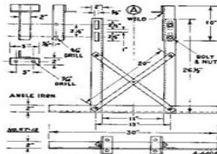
ILLUSTR. 18B. CONSTRUCTION DETAIL OF THE HOME-MADE STAND WHICH SUPPORTS THE FRONT OR ENGINE SECTION.
