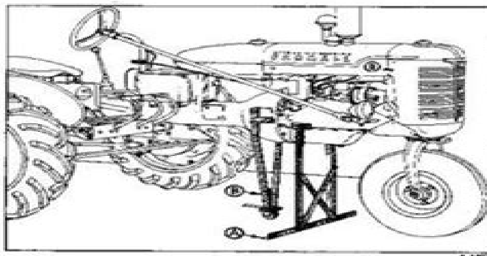
ILLUSTR. 18A. SHOWING A SIMPLE METHOD OF SUPPORTING A FARMALL A OR B TRACTOR WHILE SEPARATING THE FRONT AND REAR SECTIONS FOR THE PURPOSE OF REMOVING THE CLUTCH.
