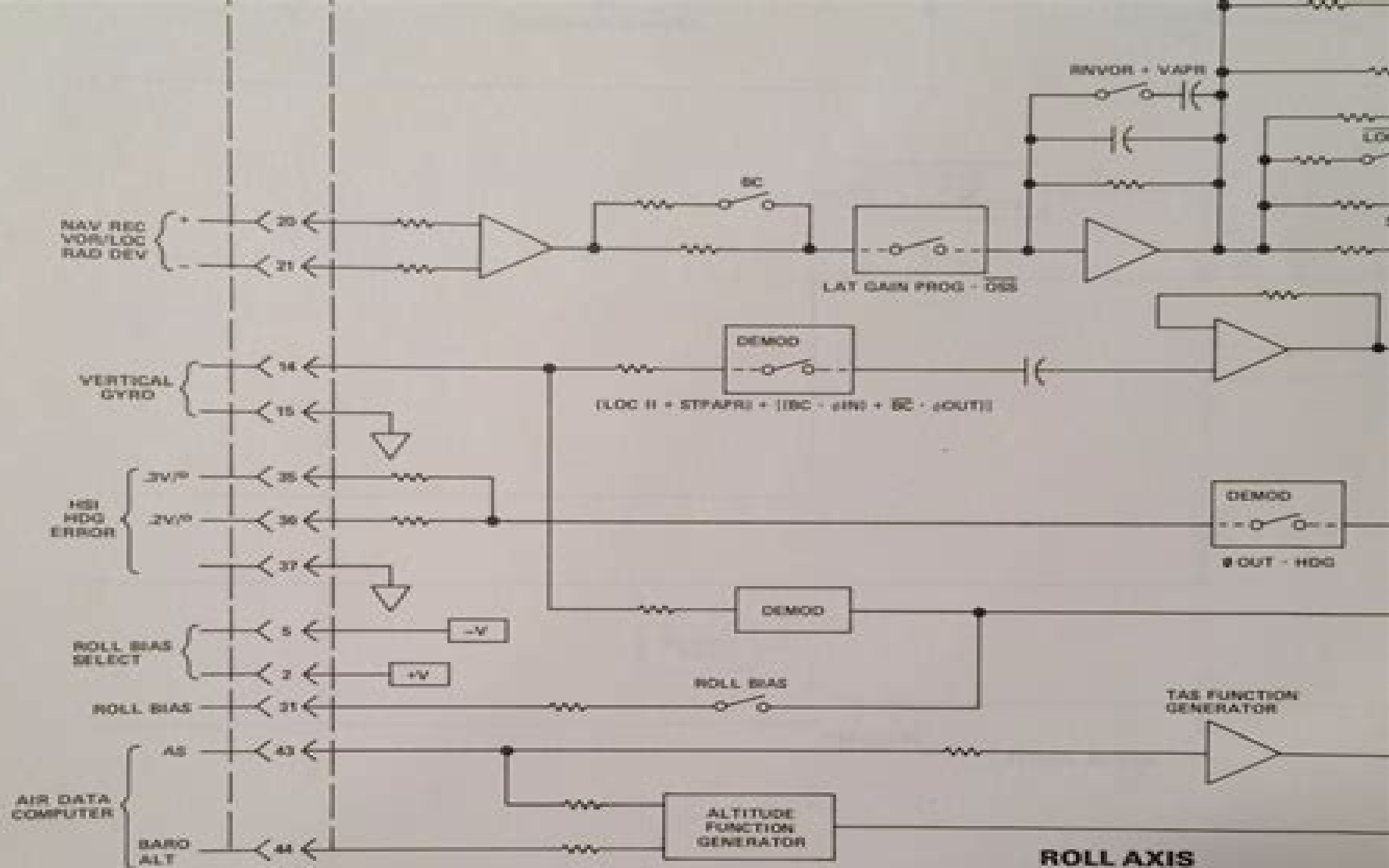
Flight Director Computer Block Diagram Figure 124 (Sheet 1 of 4)
