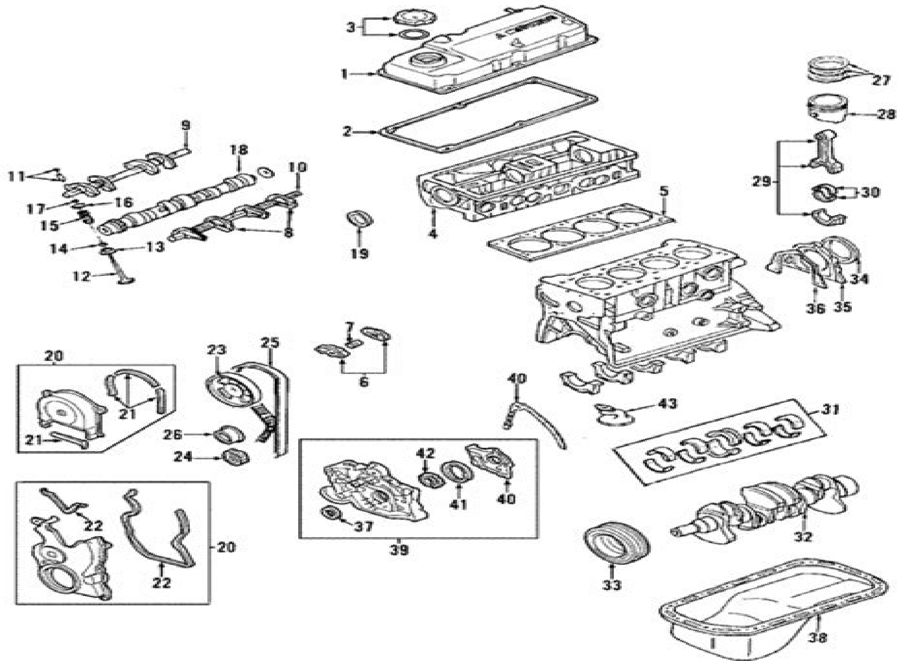
ENGINE - 4 CYLINDER, SINGLE OVERHEAD CAM
