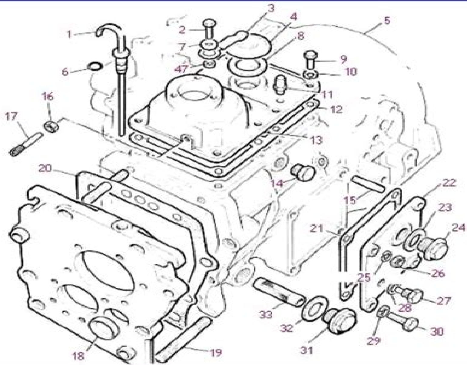
Gearbox
