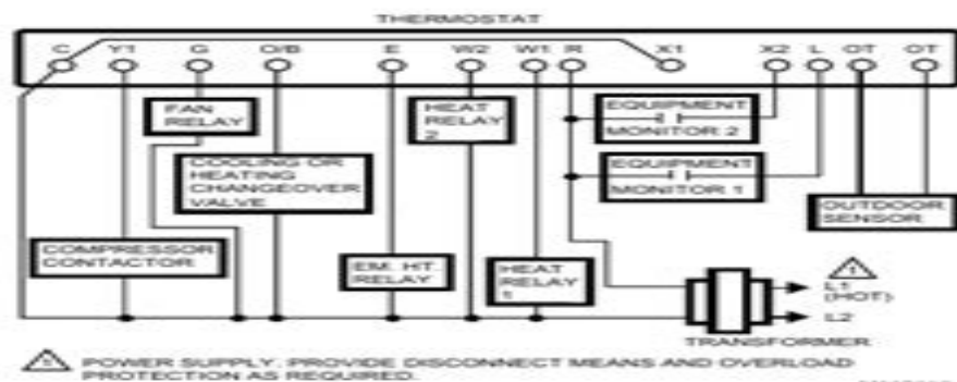
Fig. 3. Typical hookup of T8611G in a heat pump system.
