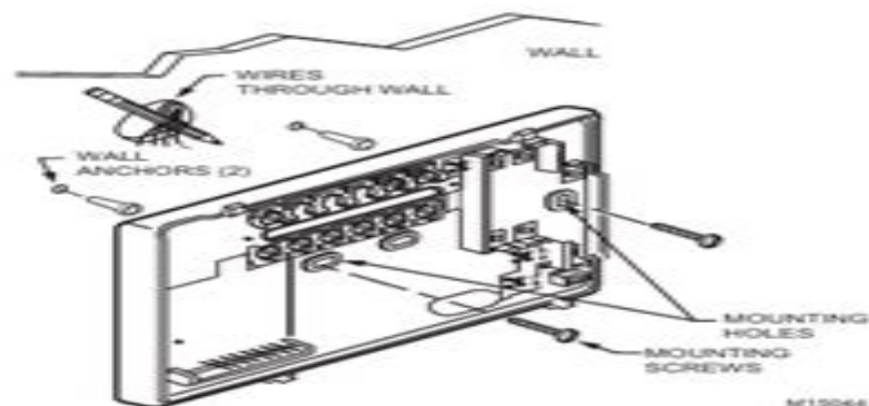
Fig. 2. Mounting the wallplate.
