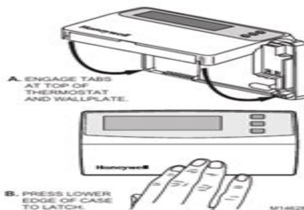
Fig. 5. Mounting thermostat on wallplate.
