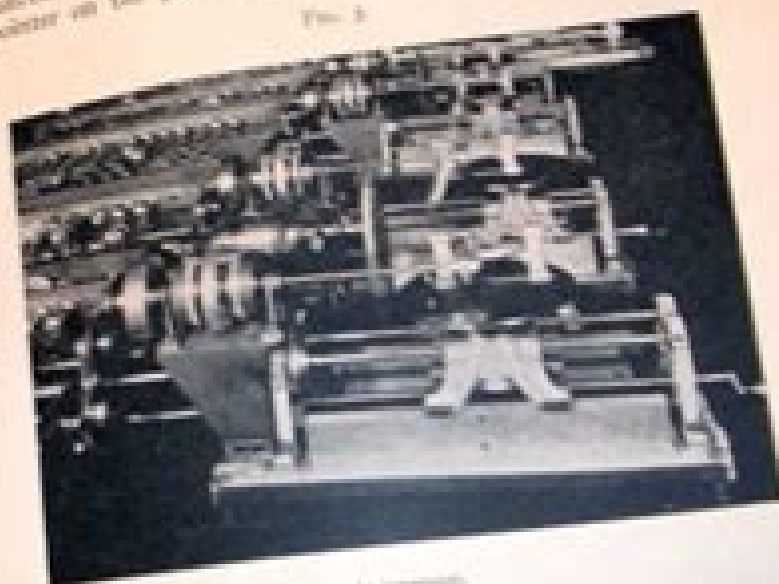
An integrator.
