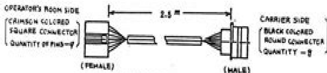
Figure 4-37. Emergency Cable
