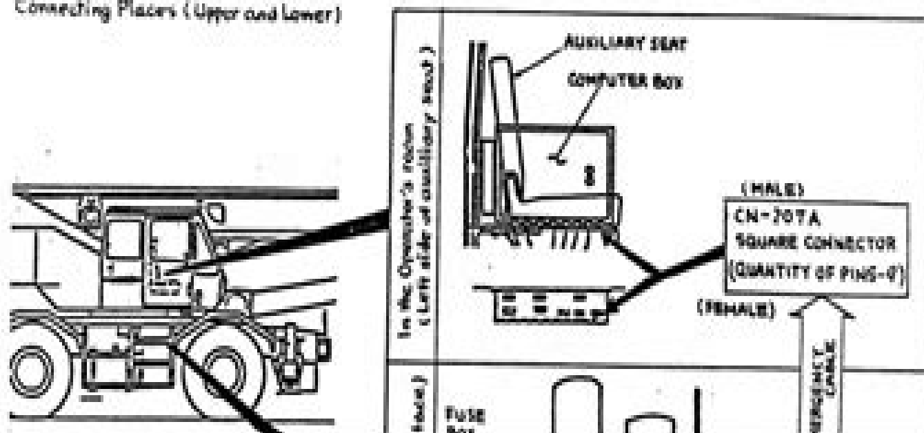
Figure 4-37. Emergency Cable
