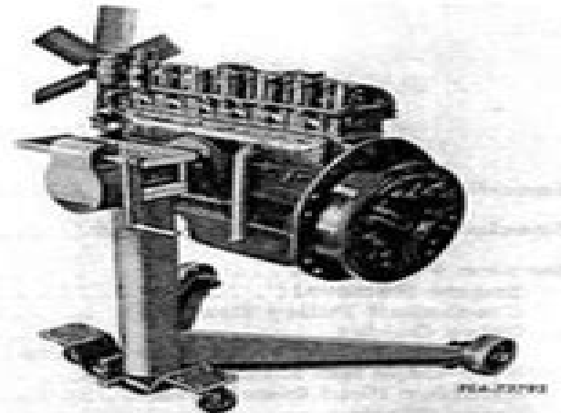
Illustr. 1-2. Engine Mounted in engine stand.
