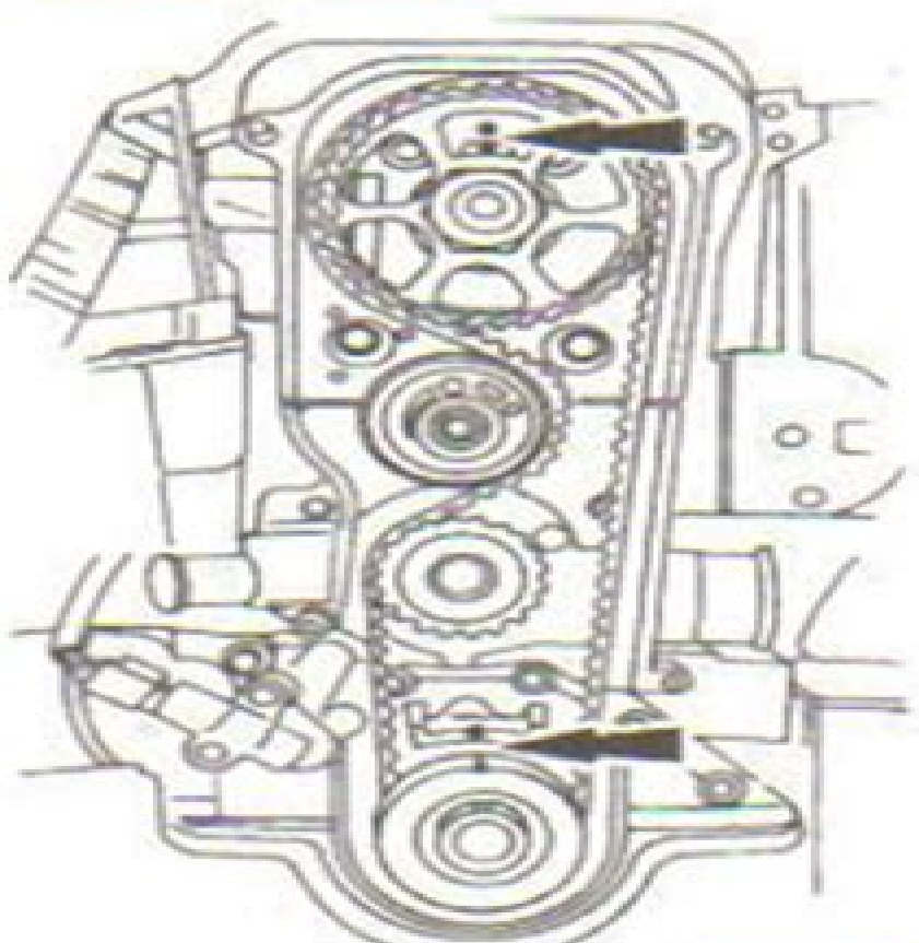
Fig. 25 Timing mark alignment
